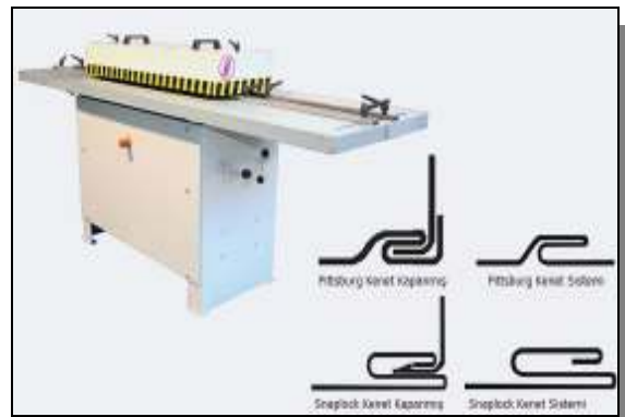
LOCK FORMING MACHINE
